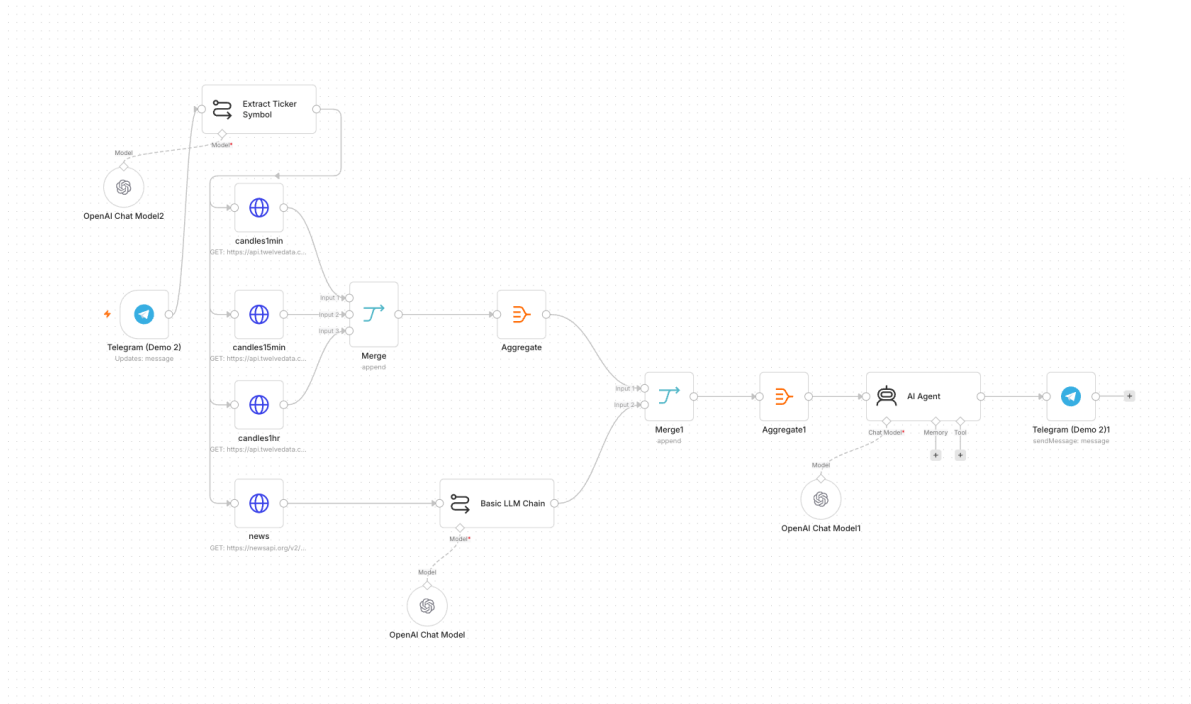
Activity 6 workflow — Finance API to Telegram day trader
